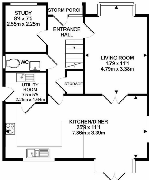
GROUND FLOOR APPROX. FLOOR AREA 666 SQ.FT. (61.9 SQ.M.)
